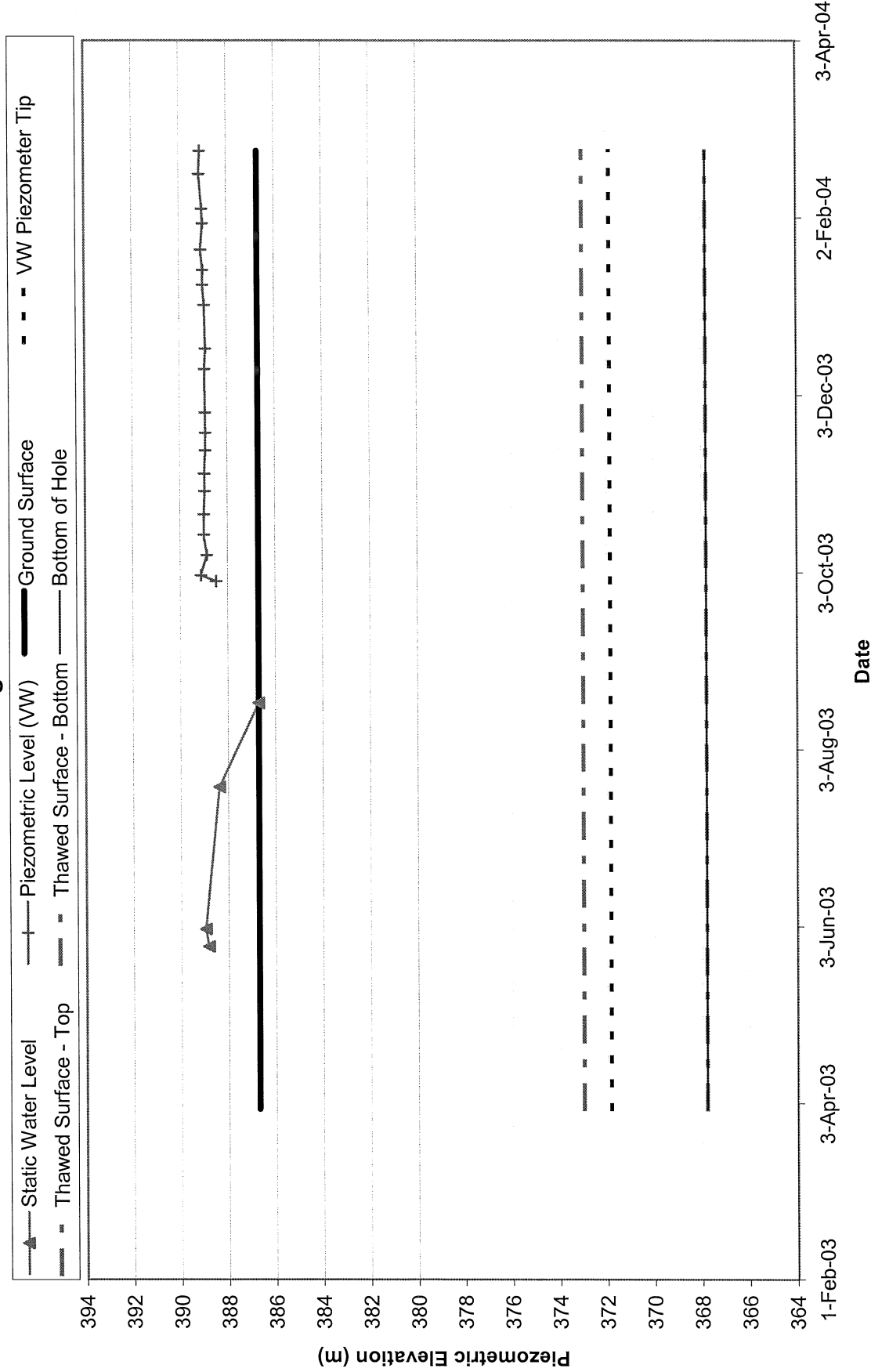
Figure III-1 Piezometer Monitoring Results for BGC03-12
