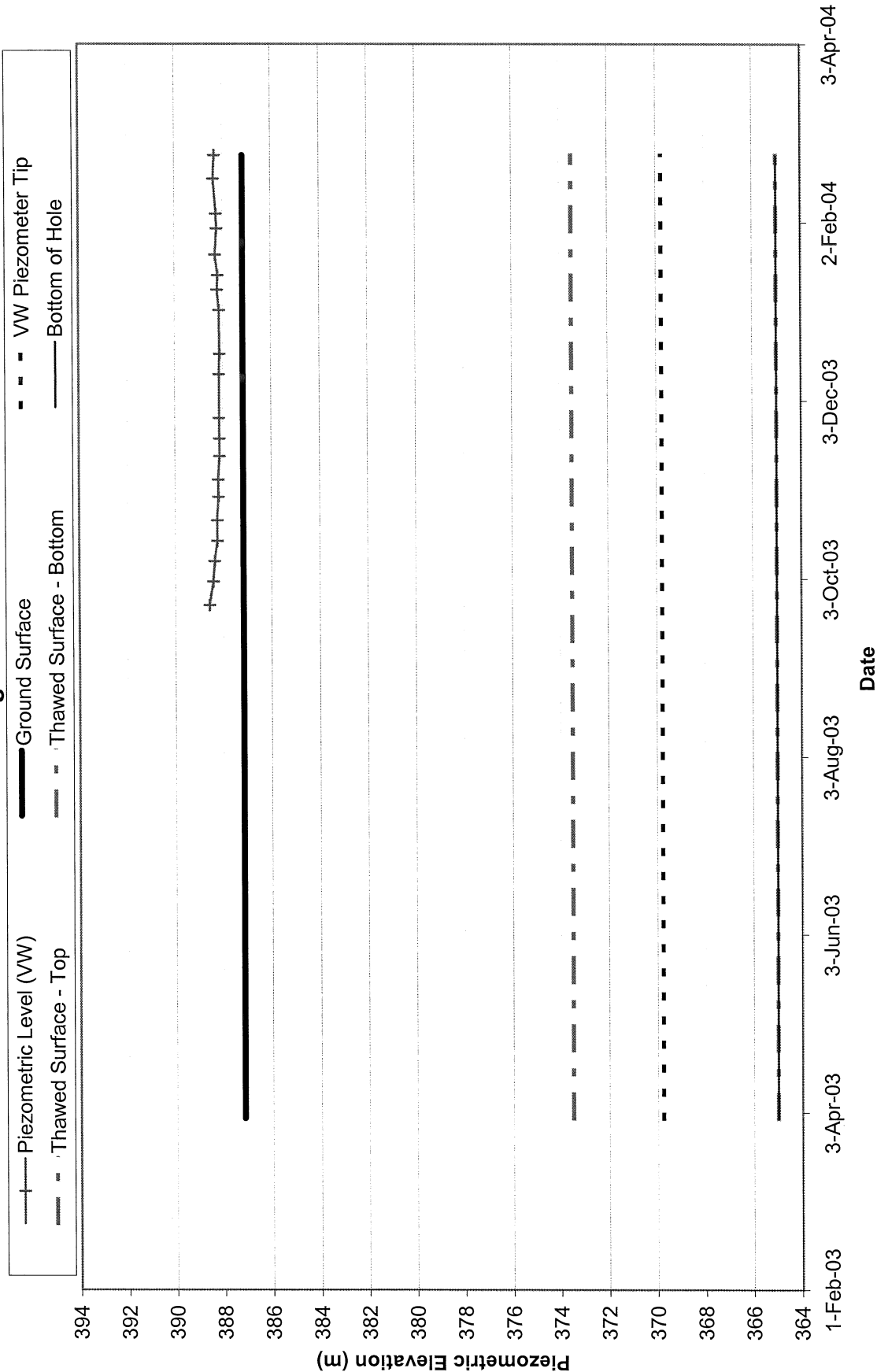
Figure III-4 Piezometer Monitoring Results for BGC03-32
